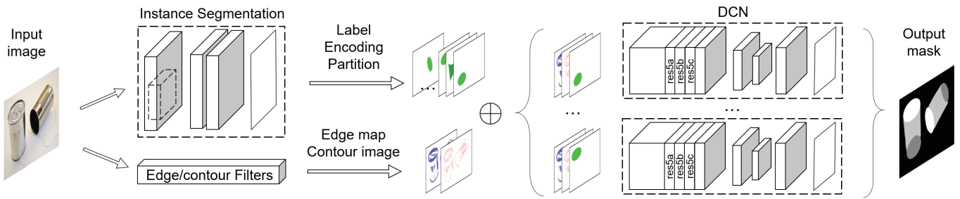
Fig. 3: The structure of our GeoNet is composed by an instance segmentation network (Mask R-CNN) and a deformable convolutional network derived from [16], [17]. The net outputs instance masks labeled as semantic parts (profiles, bodies).
